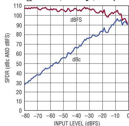
LTC2264-14: SFDR vs Input Level, f_{IN} = 70\text{MHz} , 2V Range, 40Mps
