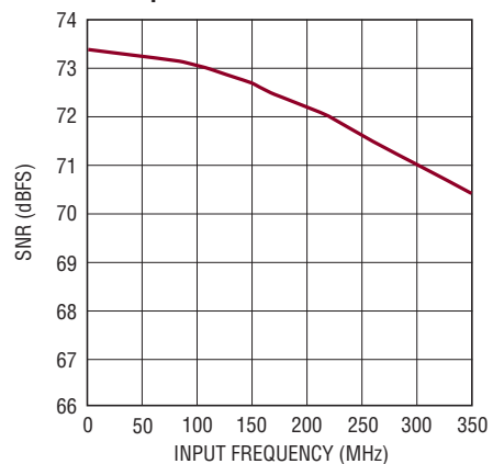
LTC2264-14: SNR vs Input Frequency, -1\text{dBFS} , 2V Range, 40Mps
