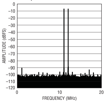
LTC2264-14: 8k Point 2-Tone FFT, f_{IN} = 68\text{MHz} , 69\text{MHz} , -1\text{dBFS} , 40Mps
