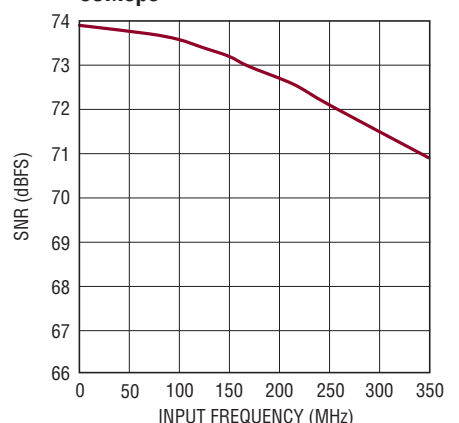
LTC2265-14: SNR vs Input Frequency, -1dBFS, 2V Range, 65Msps
