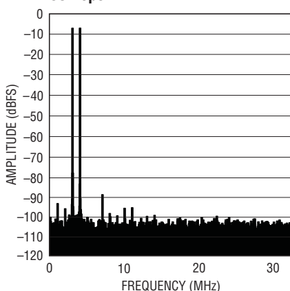
LTC2265-14: 8k Point 2-Tone FFT, f_{IN} = 68\text{MHz} , 69MHz, -1dBFS, 65Msps
