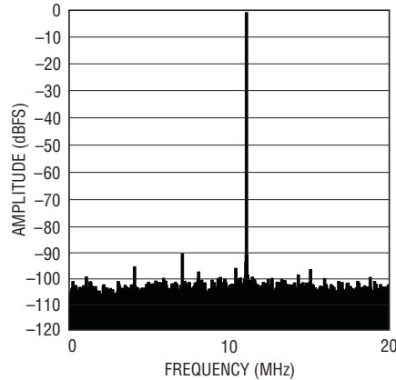
LTC2264-14: 8k Point FFT, f_{IN} = 69\text{MHz} , -1\text{dBFS} , 40Mps
