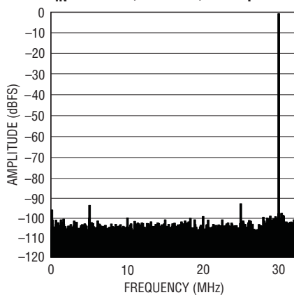
LTC2265-14: 8k Point FFT, f_{IN} = 30\text{MHz} , -1dBFS, 65Msps
