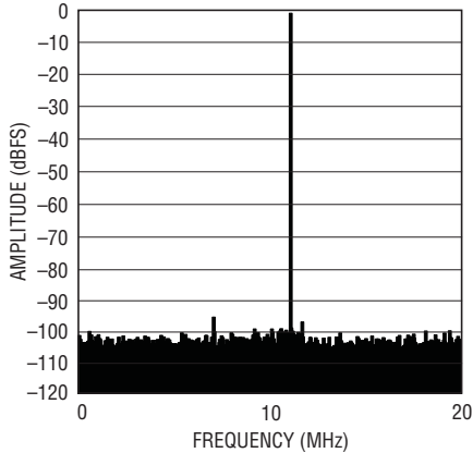
LTC2264-14: 8k Point FFT, f_{IN} = 29\text{MHz} , -1\text{dBFS} , 40Mps
