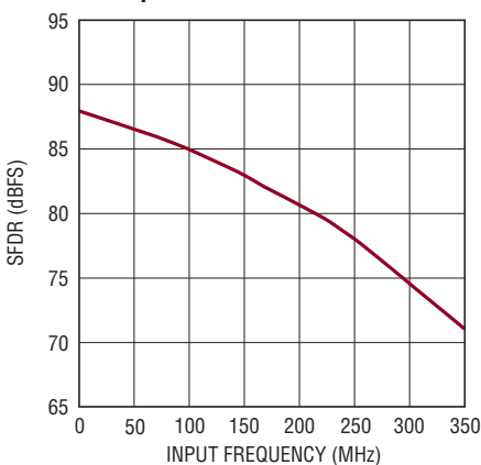
LTC2264-14: SFDR vs Input Frequency, -1\text{dBFS} , 2V Range, 40Mps
