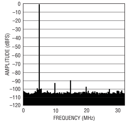
LTC2265-14: 8k Point FFT, f_{IN} = 5\text{MHz} , -1dBFS, 65Msps
