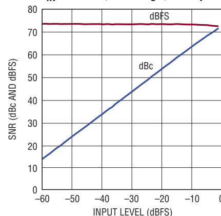
LTC2265-14: SNR vs Input Level, f_{IN} = 70\text{MHz} , 2V Range, 65Mps
