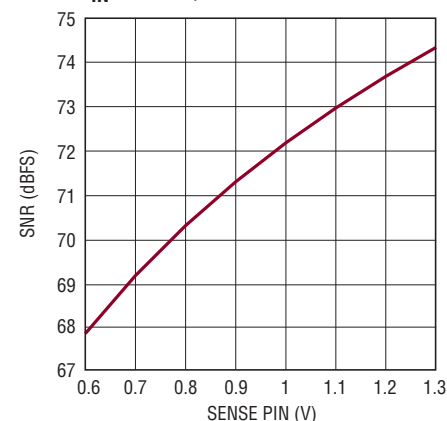
LTC2265-14: SNR vs SENSE, f_{IN} = 5\text{MHz} , -1dBFS
