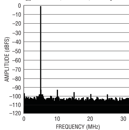
LTC2265-14: 8k Point FFT, f_{IN} = 70\text{MHz} , -1dBFS, 65Msps
