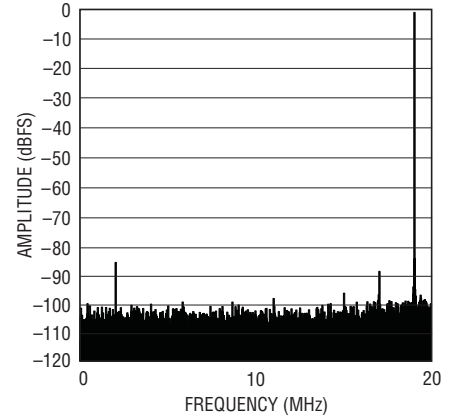
LTC2264-14: 8k Point FFT, f_{IN} = 139\text{MHz} , -1\text{dBFS} , 40Mps
