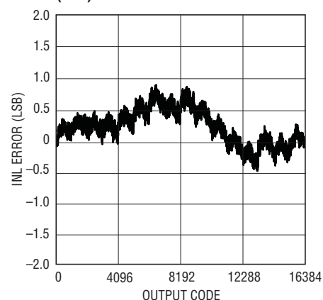
LTC2264-14: Integral Nonlinearity (INL)
