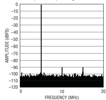
LTC2264-14: 8k Point FFT, f_{IN} = 5\text{MHz} , -1dBFS, 40Mps
